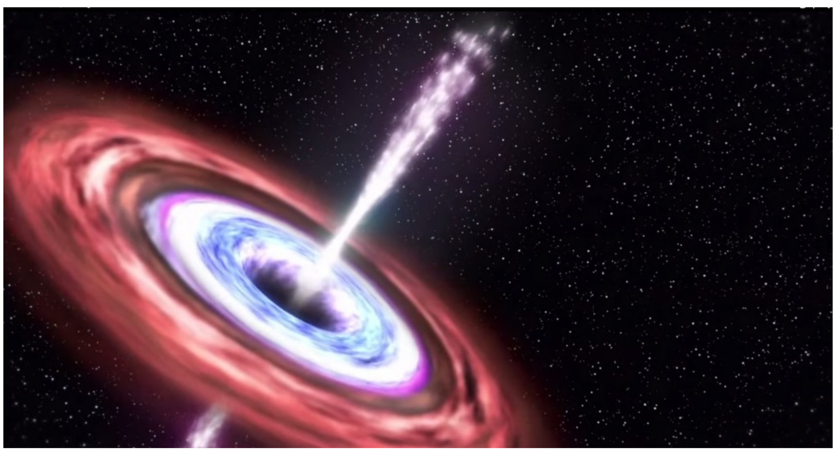
(http://blog.seagate.com/wp-content/uploads/2015/03/NASA-illustration-accretion-disk-around-a-black-hole-powering-a-particle-jet.jpg)
